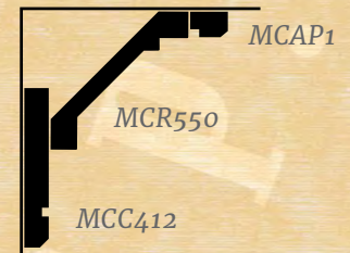
MCR550 MCAP1, MCC412
