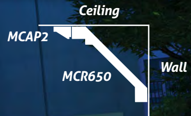
MCR650 Step on Ceiling, MCAP2
