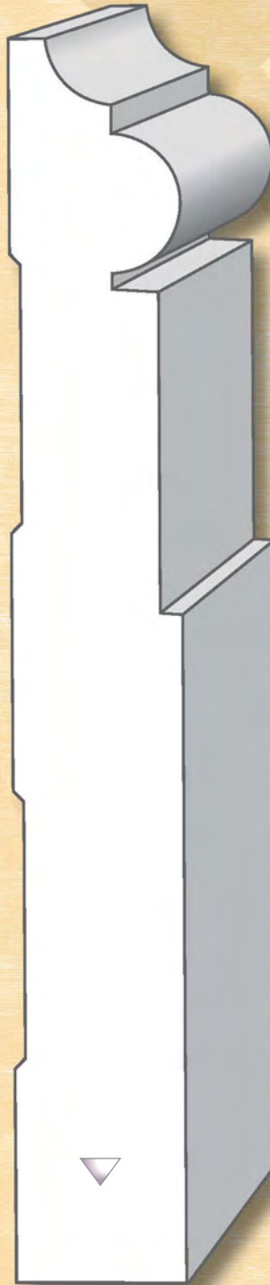
DCB714 1 x 7-1/4 18' Lengths
