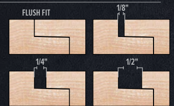
fit detail
